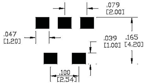
PCB FOOTPRINT
